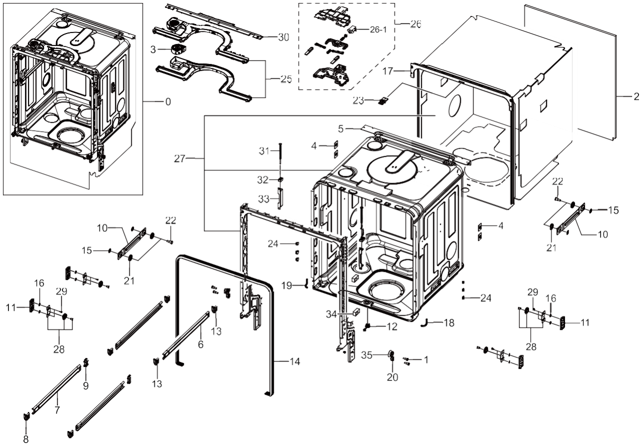
Assy Door Parts List
