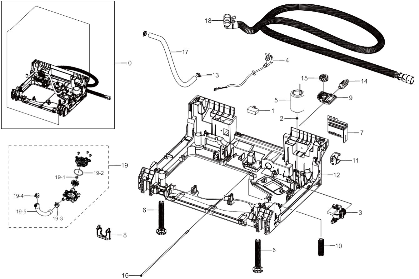
Assy Base Parts List
